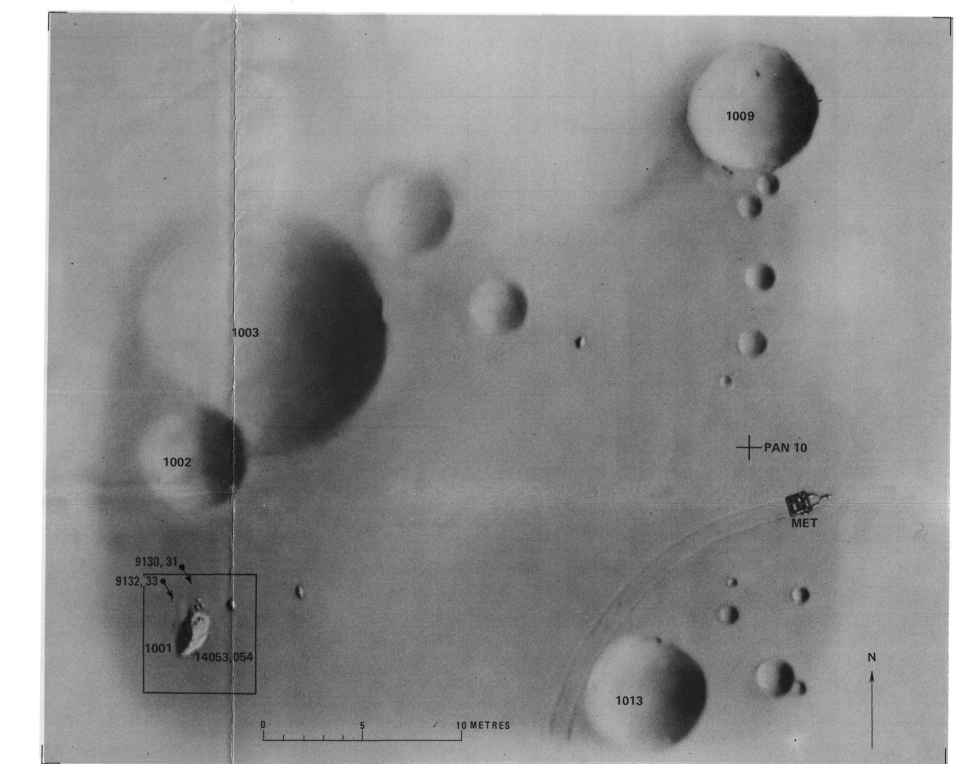
SHADED RELIEF MAP OF STATION B3
