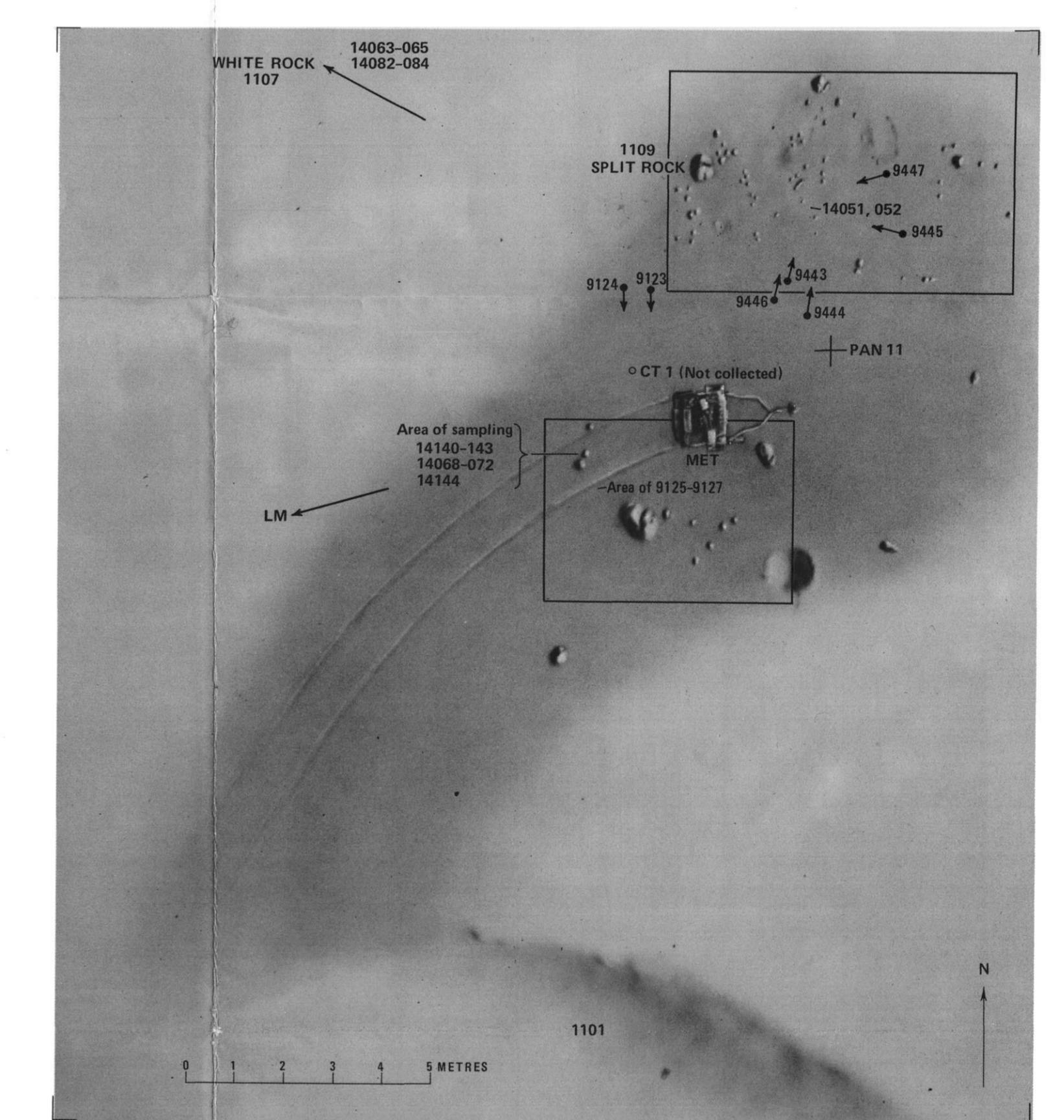
SHADED RELIEF MAP OF STATION C'
