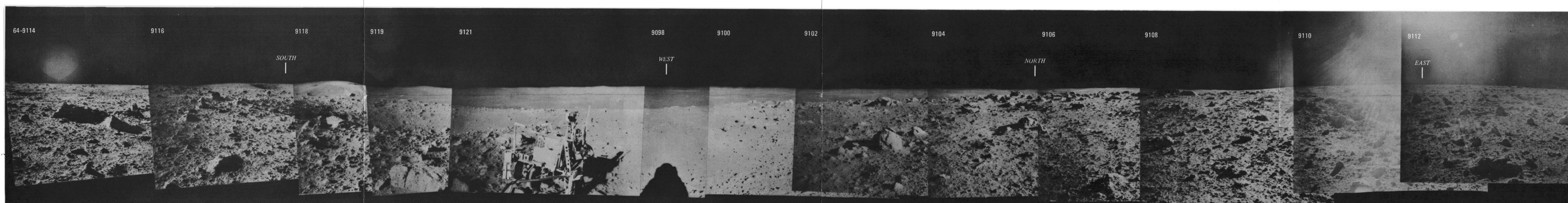
PANORAMA 11, TAKEN AT STATION C'
