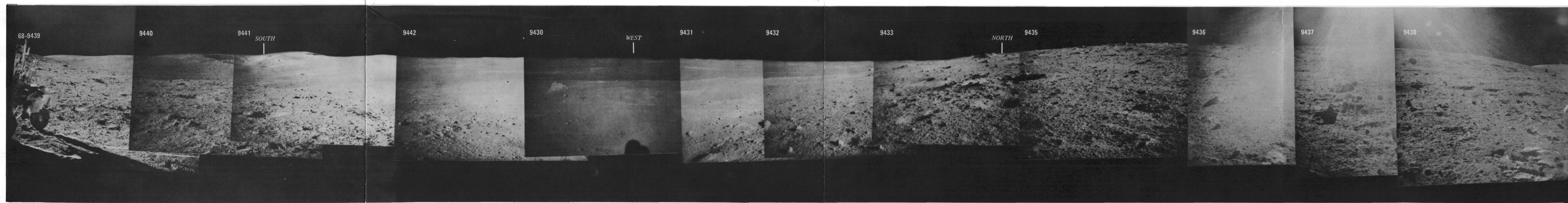
PANORAMA 10, TAKEN AT STATION B3
