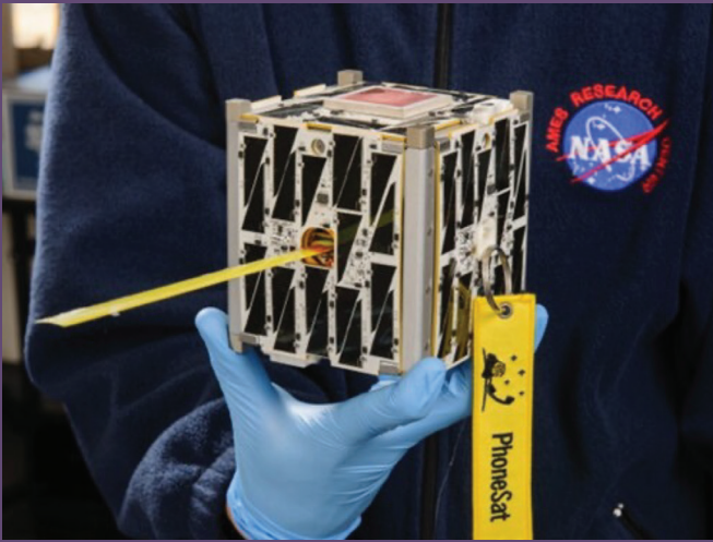
NASA's PhoneSat, a four-by-four-inch CubeSat satellite, uses an Android smartphone as its motherboard. It was among the 29 satellites launched from Wallops Island, Virginia. Another miniature satellite, developed by high school students, was also on board. Credit: NASA. Credit: Dominic Hart/AP.
