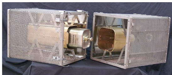
Space Station Backup Oxygen Candle System (4" x 4" square candle)
