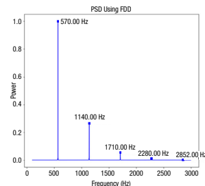
Figure 2c: Bellows MM Data
