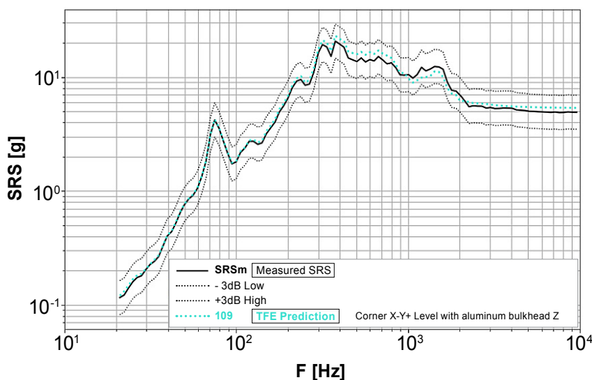
Finite element model of notional satellite (above) and its SRS using this TFE shock prediction methodology (right)
