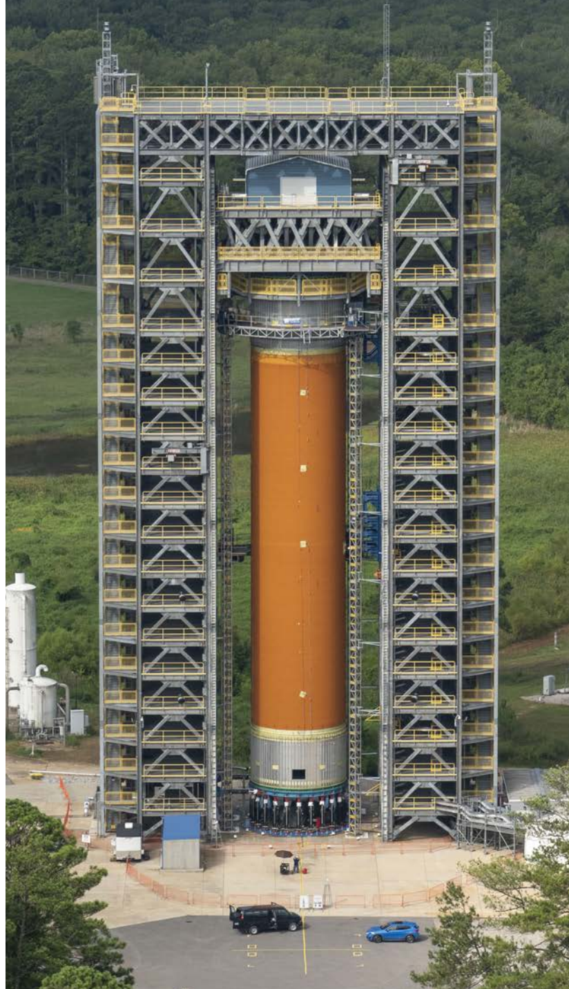
Aerial photograph of MSFC test stand 4693 with the Liquid Hydrogen test article (LH2) in the stand. (NASA/MSFC/Fred Deaton)
