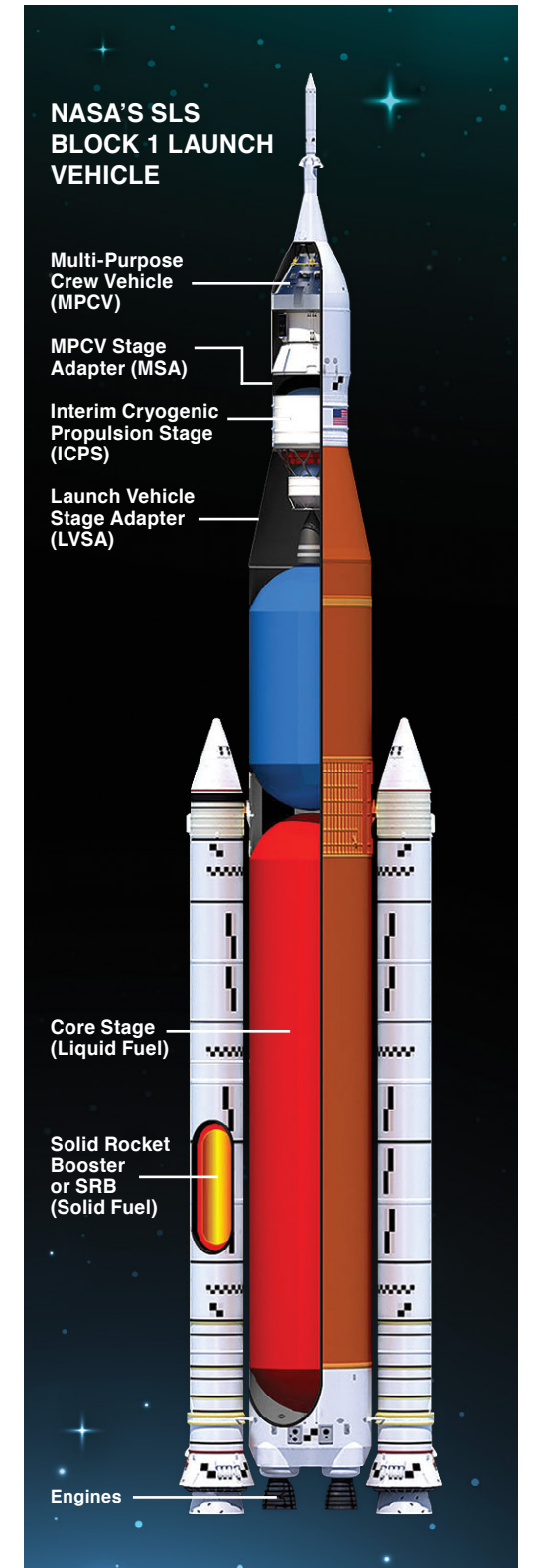
Figure 1. Integrated SLS stacked system.
