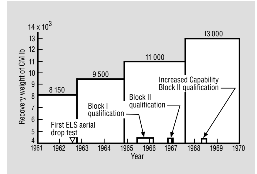
The Apollo crew module mass increased by almost 60% before the final configuration was qualified for flight, having significant impact on the design and qualification of the Earth landing system (ELS).
