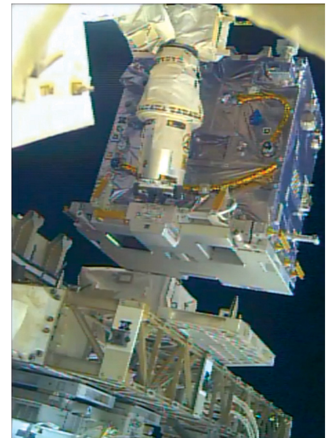
The RRM3 fluid transfer module during installation on the International Space Station External Logistics Carrier.
