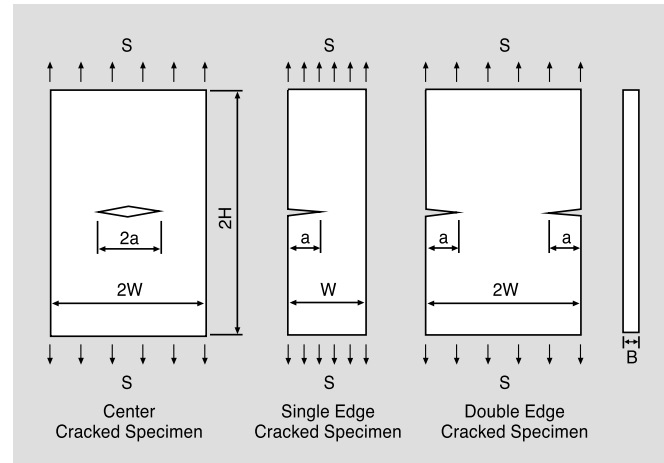
Different specimens analyzed for verifying J-A prediction methodology.
