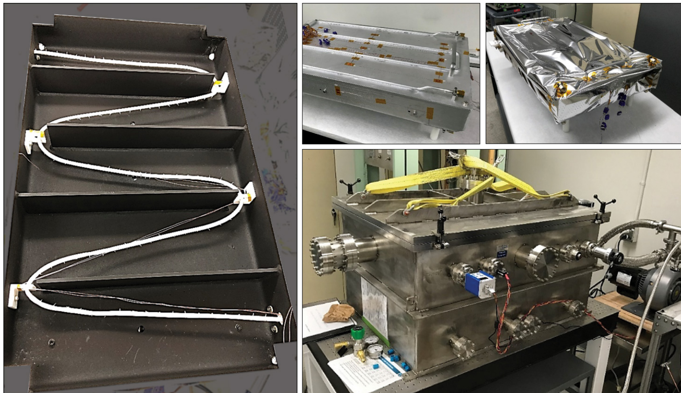
Clockwise from left: A wire bundle test article is placed in a temperature-controlled shroud, then insulated, and finally sealed in a chamber for ampacity/temperature rise measurements as current is applied in air or under vacuum conditions.
