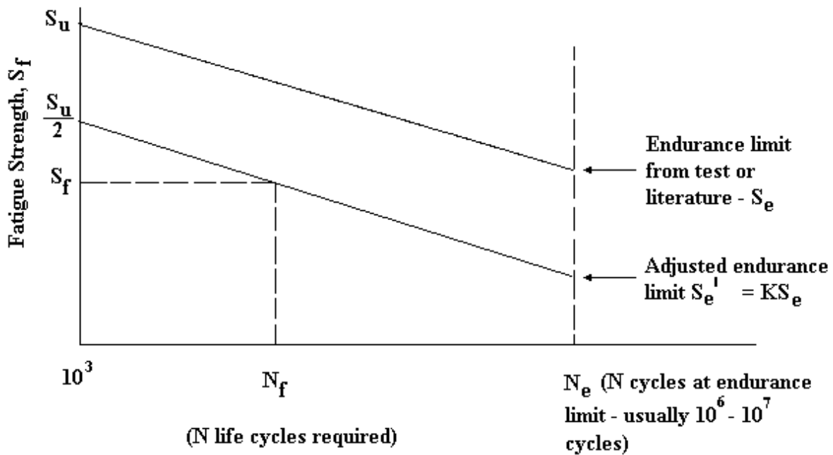
Linearized Fatigue Curve
