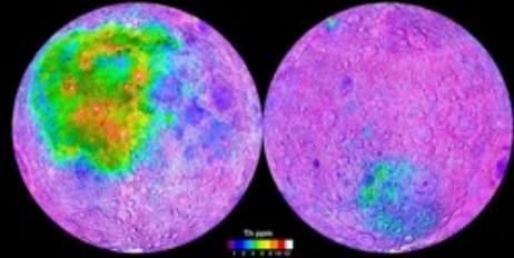
Indication of where KREEP is (Procellerum KREEP Terrane)
