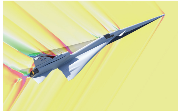
Computer simulation showing how shock waves move away from the X-59 as it flies faster than sound. The pattern is different from the way shock waves from a conventional supersonic aircraft come together to produce a sonic boom. Instead, the X-59 will produce a quieter sonic thump. Credit: NASA
