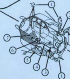
KVANT-1 ASTROPHYSICS MODULE – 37KE 30 Mar 1987 6.3 m × 4.36 m 11,000 kg 40.0 cu m
