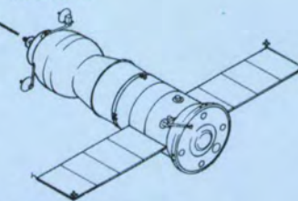
PROGRESS RESUPPLY TRANSPORT Payload 2400 kg Spacecraft 7320 kg 7.23 m × 2.72 m, 10.6 m Across Solar Arrays
