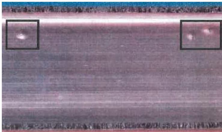
Figure 1: Hydrogen Blisters on Al 6061 T6511.
