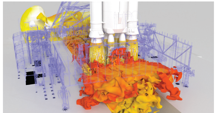
Ames produced a visualization of SLS exhaust gas flow during liftoff from Launch Complex 39B to accurately understand how liquid and gases flowing during launch can cause various kinds of waves at the launch pad.
