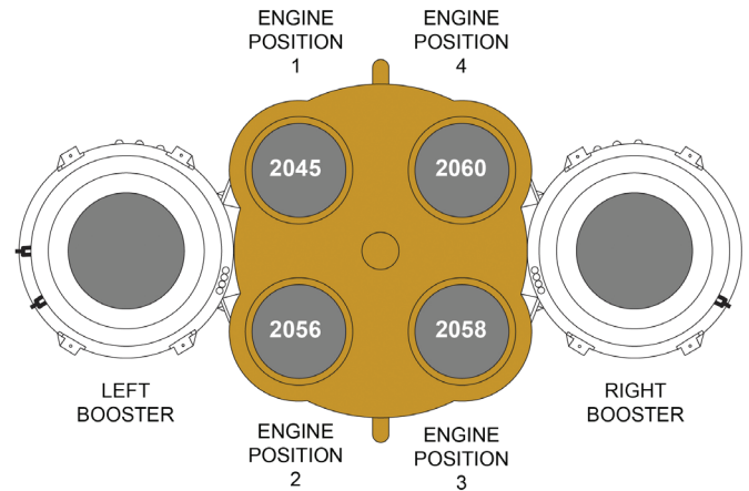
RS-25 ORIENTATION VIEW LOOKING UP FROM THE BOTTOM Artemis engine serial numbers and their position in the core stage relative to the boosters.
