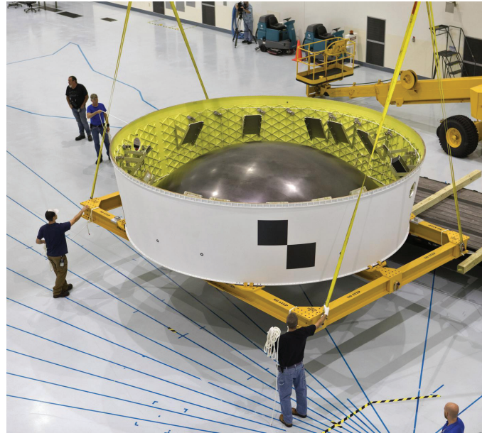
The completed Orion stage adapter after delivery from Marshall to Kennedy. The brackets to hold the dispensers for the CubeSat payloads and avionics unit are visible.
