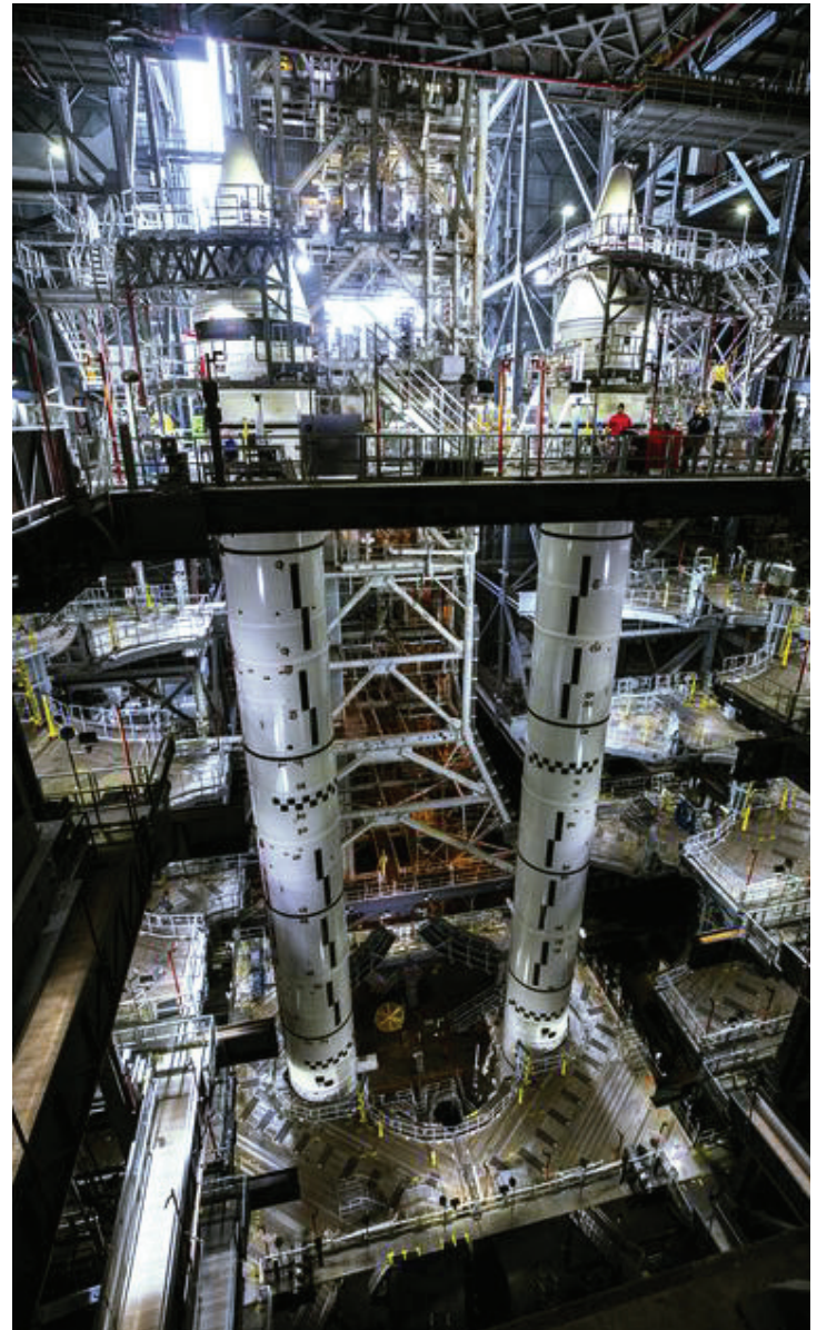
The completed Artemis I boosters are shown stacked on the mobile launcher in the Vehicle Assembly Building at Kennedy Space Center before integrating the other elements of SLS and Orion.
