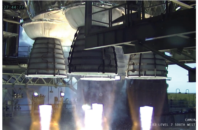
The Artemis I RS-25 liquid fuel engines operated successfully as part of the core stage Green Run hot fire test at Stennis in early 2021.
