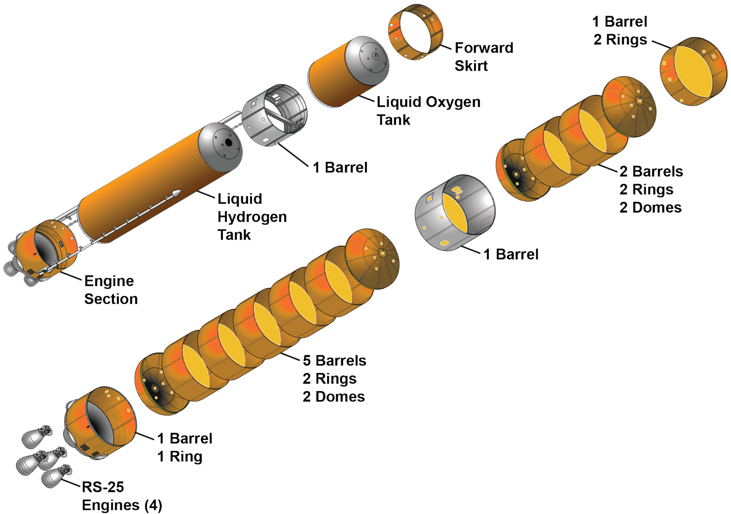
The SLS core stage is comprised of 10 barrel sections, four dome sections, and seven rings as shown in this illustration of the core stage major components.
