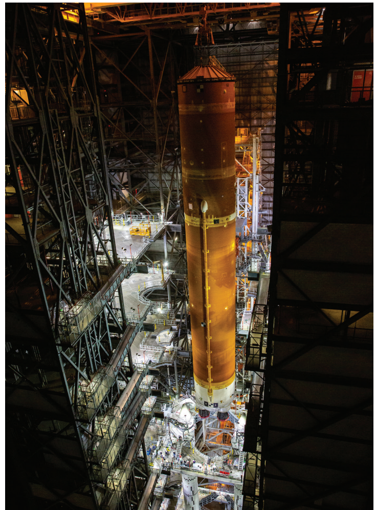
The SLS core stage, the tallest rocket stage NASA has ever built, is lowered between the Artemis I boosters in the Vehicle Assembly Building.
