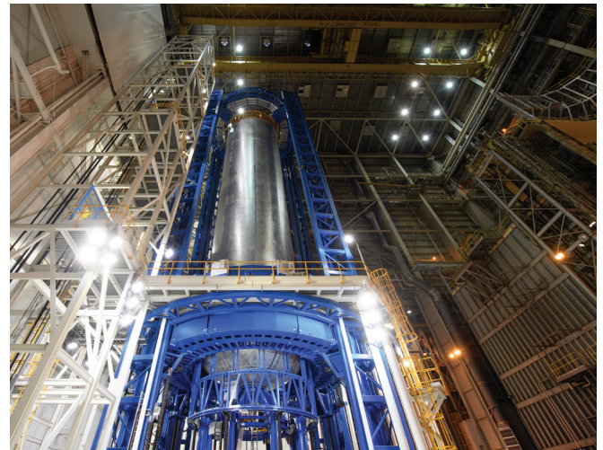
The Vertical Assembly Center at Michoud is one of the world's largest welding tools and is used to execute vertical friction-stir welds of the SLS core stage liquid hydrogen tank.
