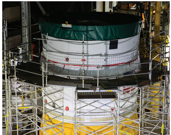
The ring-shaped Orion stage adapter is filled with 10 shoebox-sized CubeSats that will deploy when the ICPS separates from Orion on its way to the Moon.
