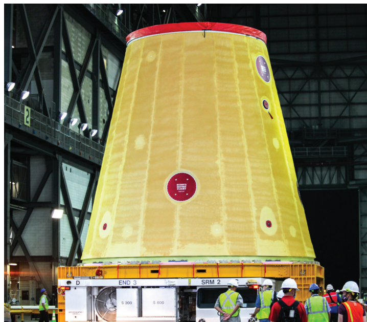
The Artemis I launch vehicle stage adapter arrives at the Vehicle Assembly Building for stacking on the Artemis I rocket.
