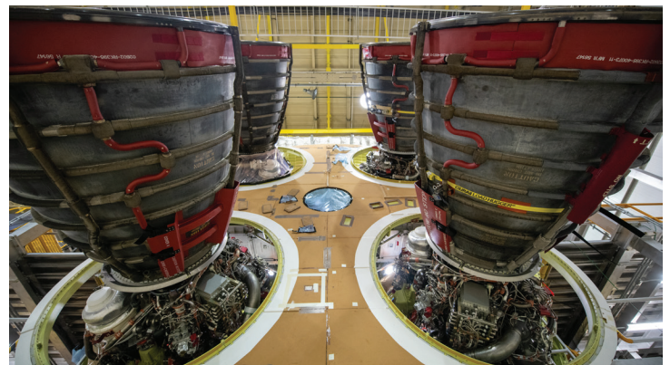
The Artemis I RS-25 engines installed in the core stage during assembly at NASA's Michoud Assembly Facility in New Orleans.
