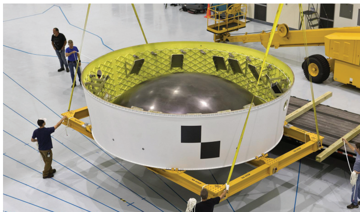
Orion stage adapter complete and ready for CubeSats.
