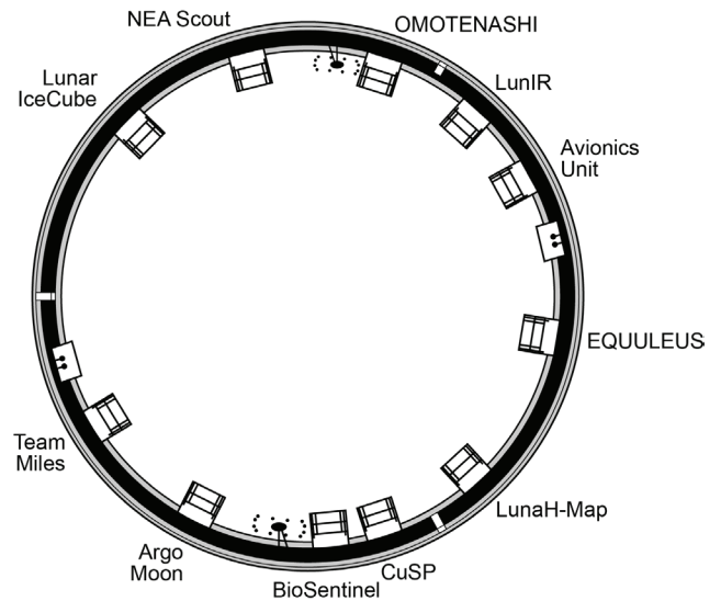
Payload berth locations on the Orion stage adapter.
