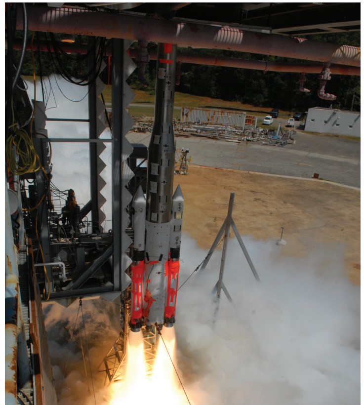
A five-percent scale model of SLS undergoes acoustic testing in 2014 at Marshall.
