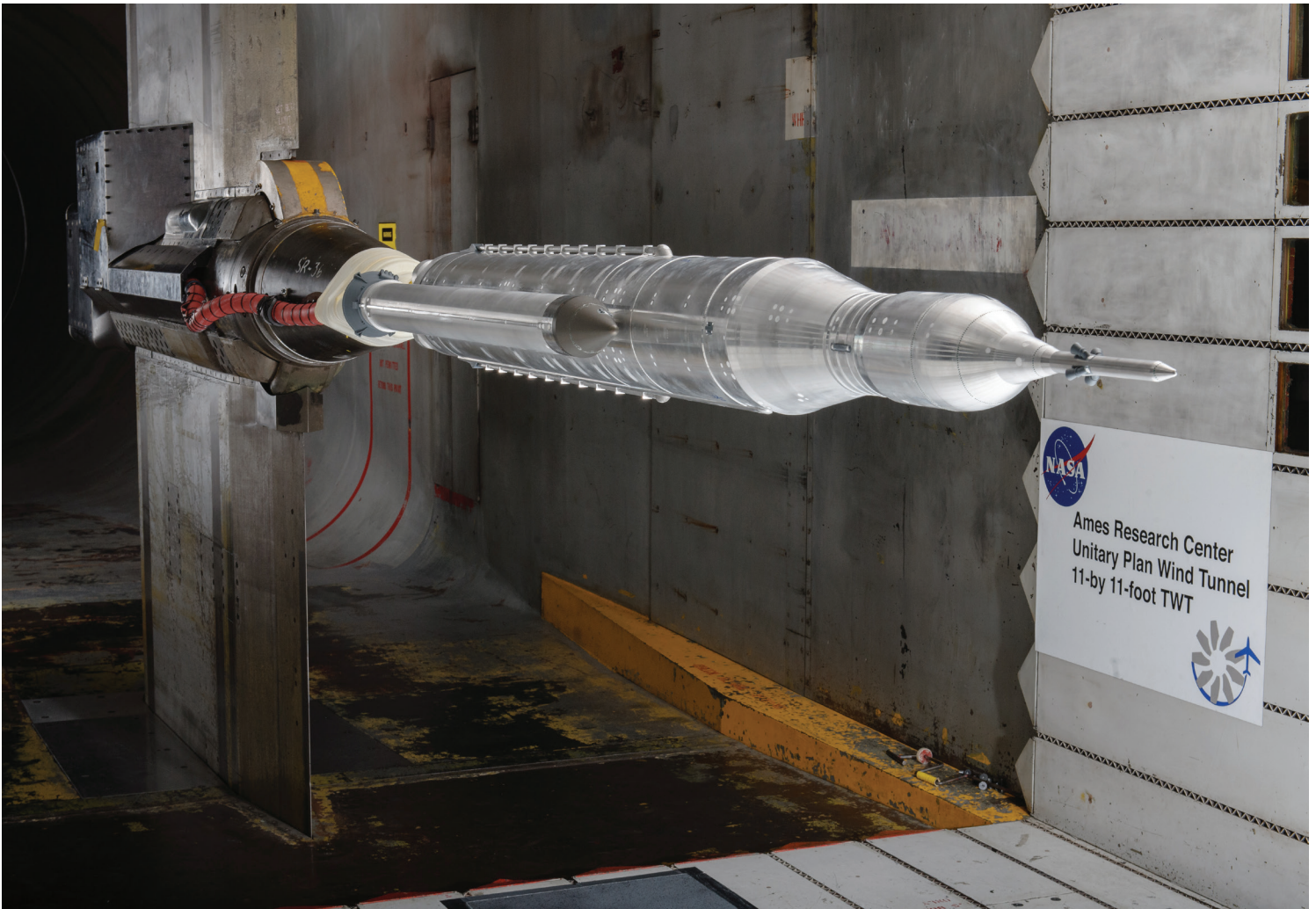
A scale model of SLS was tested in an 11-by 11-ft. (3.4-by 3.4-m) Transonic Wind Tunnel at Ames. Data from the wind tunnel tests at Ames and Langley was used to improve the design and stability of SLS.
