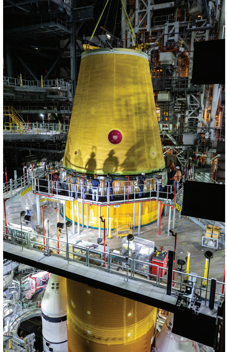
Jacobs crews bolt the launch vehicle stage adapter to the SLS core stage in the Vehicle Assembly Building.
