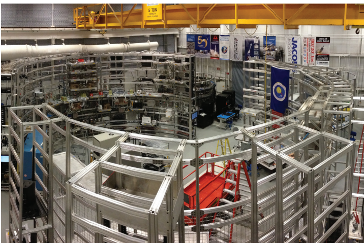
The Systems Integration Lab/Systems Integration Test Facility at Marshall is a full-scale mockup of flight-like avionics systems for the solid rocket boosters and core stage where engineers can test hardware and software integration prior to manufacture and flight.
