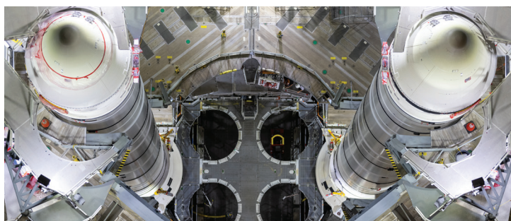
Artemis I five-segment solid rocket boosters stacked on the mobile launcher.
