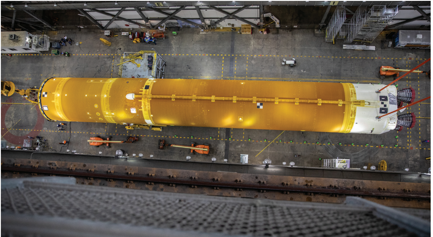
The 212-ft. (64.6 m) core stage for Artemis I in the transfer aisle of the Vehicle Assembly Building in preparation for lifting and integration on the mobile launcher. Manufactured by Boeing at Michoud, the stage houses the four RS-25 engines, propellant tanks, and flight computers. Too large to ship over land, NASA's barge Pegasus transported the Artemis I core stage to Stennis for a 'Green Run' test campaign and then to Kennedy for integration with the rest of the vehicle.
