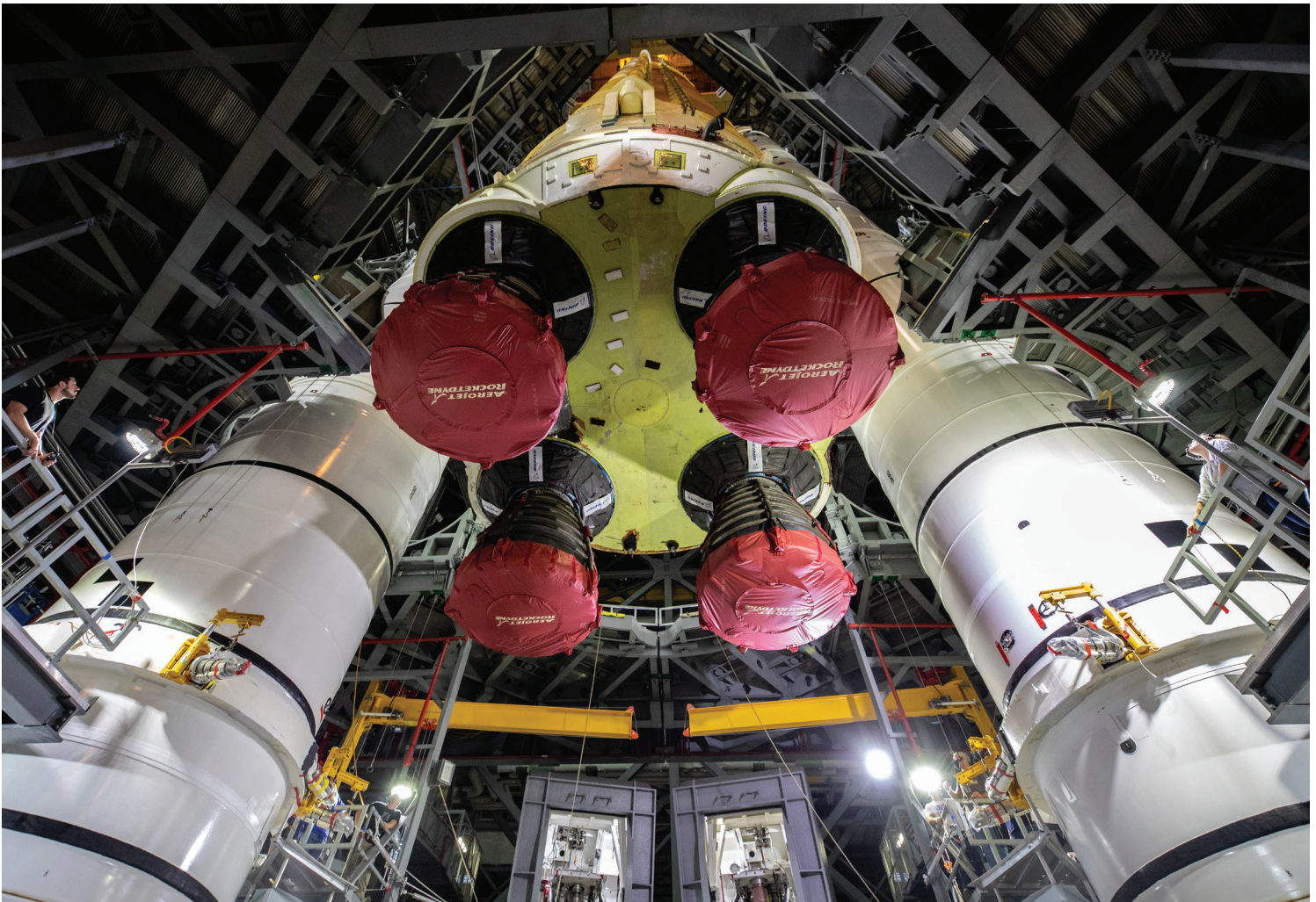
The Artemis I core stage is lowered between the SLS solid rocket boosters in the Vehicle Assembly Building. The SLS design uses a proven propulsion system of solid rocket boosters and liquid-fuel RS-25 engines to launch more payload to the Moon than any rocket since the Saturn V.
