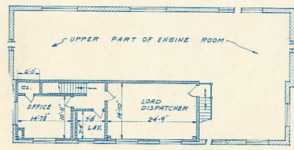
MEZZANINE FLOOR PLAN
