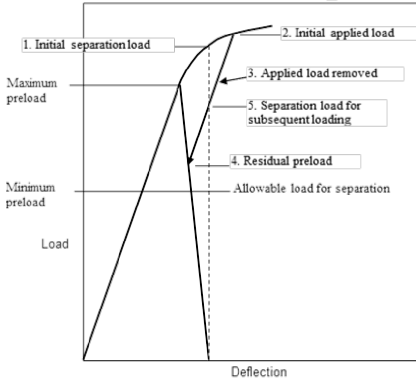
Figure 20—Fastener Yielding under an Applied Load that Exceeds the Separation Load
