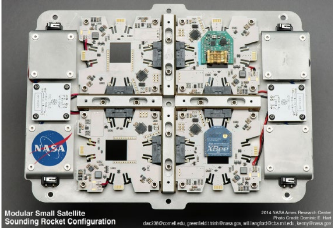
Figure 2: The OuroboroSats boards in the sounding rocket configuration. In order to conform to the low vertical clearance, the boards were arranged in a 2D array.
