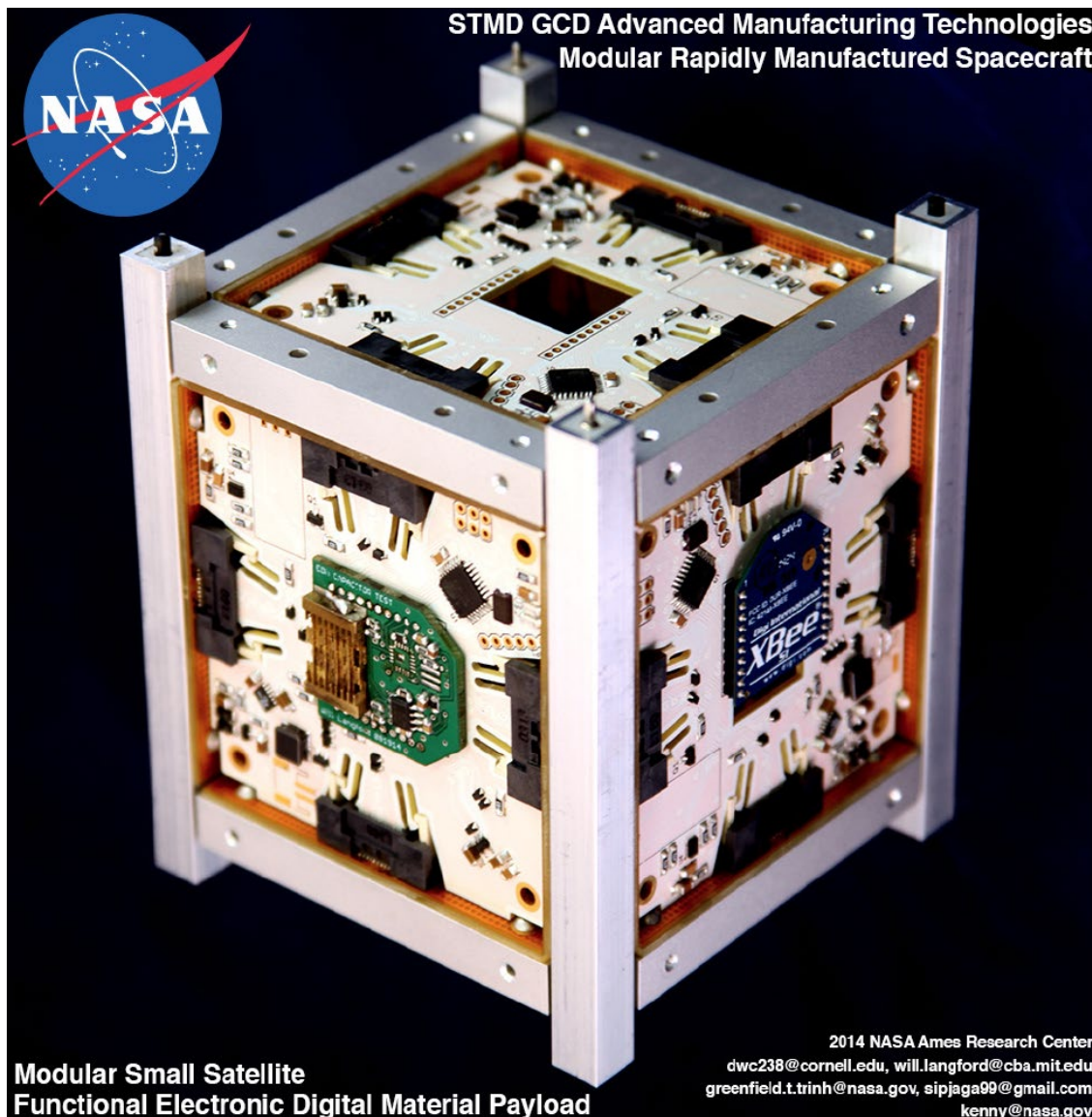
Figure 1: Six OuroboroSAt boards arranged in a cube. This configuration conforms to the CubeSat specification with regards to the overall dimensions and limit-switch placement.
