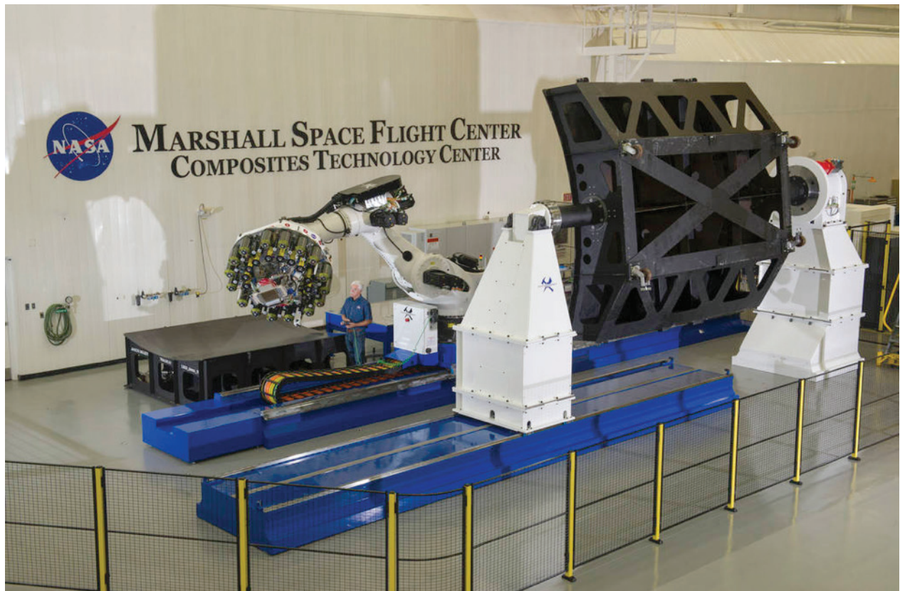
This new robotic fiber placement tool can drastically reduce the cost and improve the quality of large space structures.
