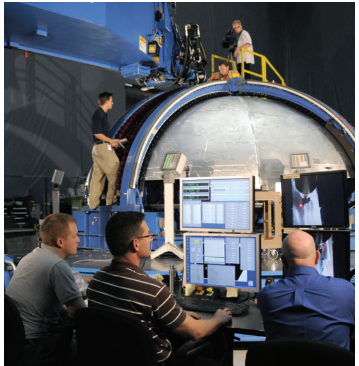
Marshall's Robotic Weld Tool can handle the complex curvatures needed for launch vehicle fuel tank domes.
