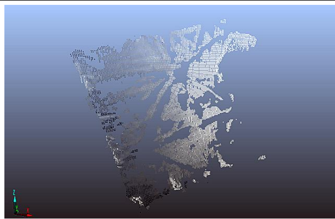
Figure V.B.10. FARO TOF ranger image of aluminized Mylar covered section of 3 meter sphere.
