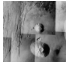
Image 3. Martian volcanoes and fault lines.
