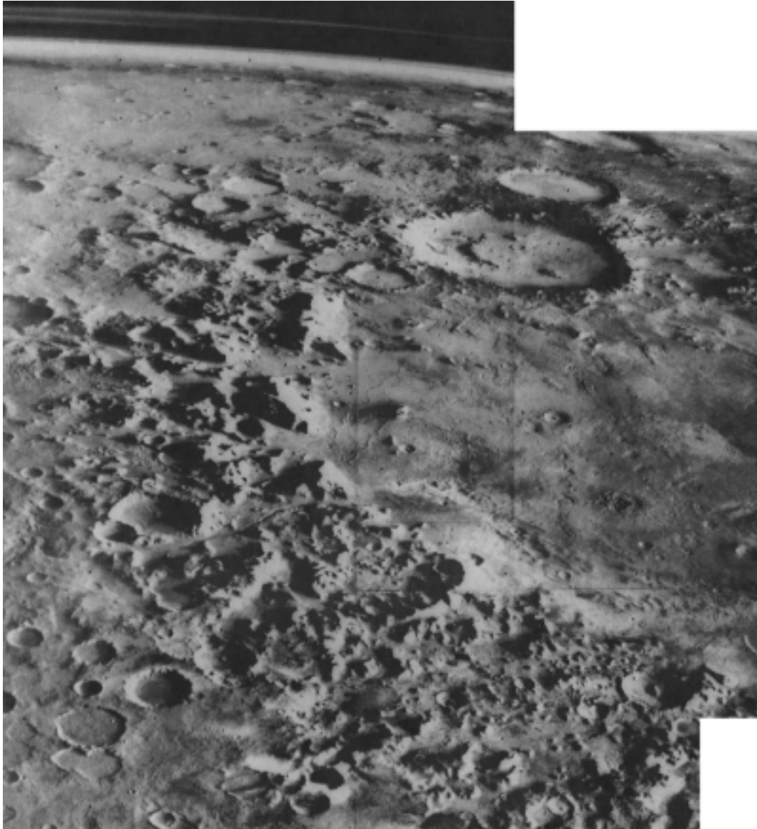
Image 2. A view across the Argyre Planitia. Scale: The large crater in the upper right is about 200 km in diameter.
